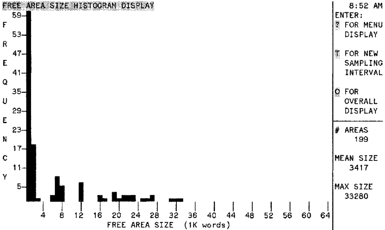
Figure 7-10. Free Area Size Histogram Display
