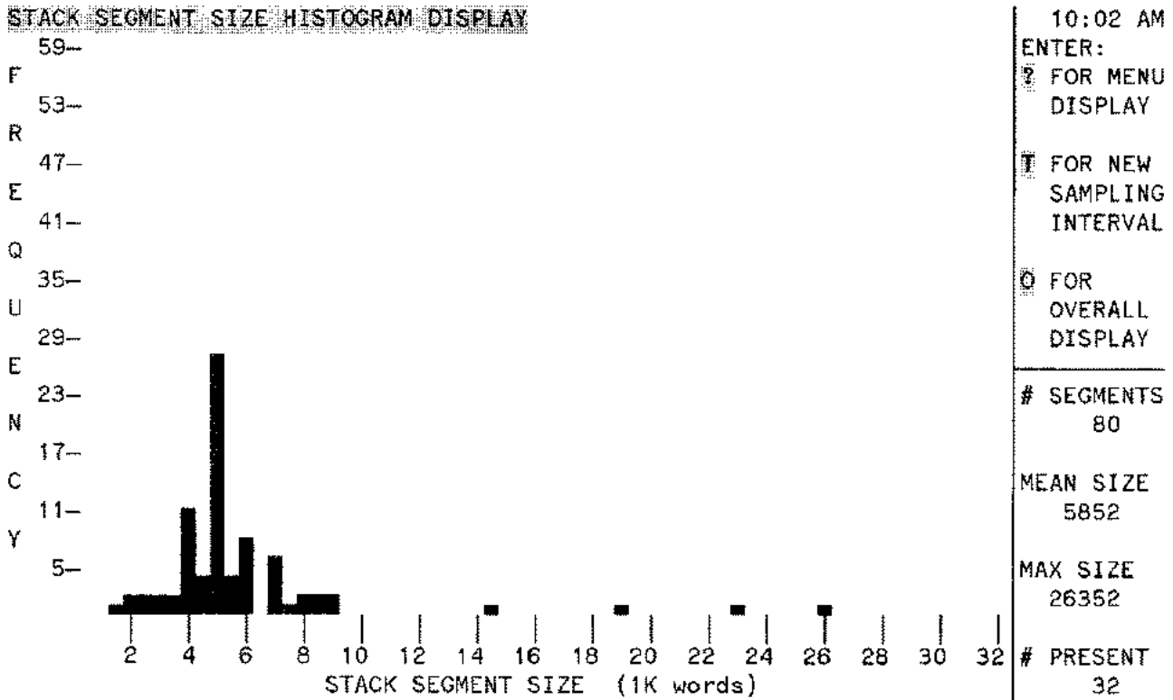
Figure 7-9. Stack Segment Size Histogram Display
