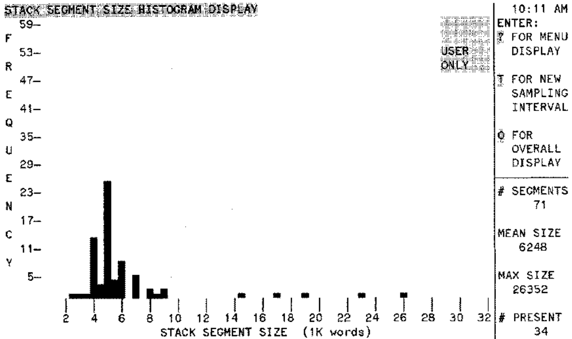
Figure 7-14. Stack Segment Size Histogram Display (user segments)
