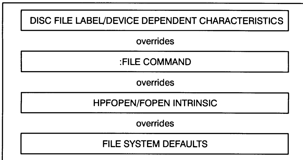
Figure 5-1. File System Hierarchy of Overrides
