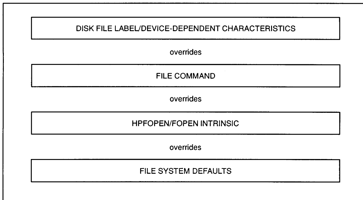
Figure 2-1. File System Hierarchy of Overrides
