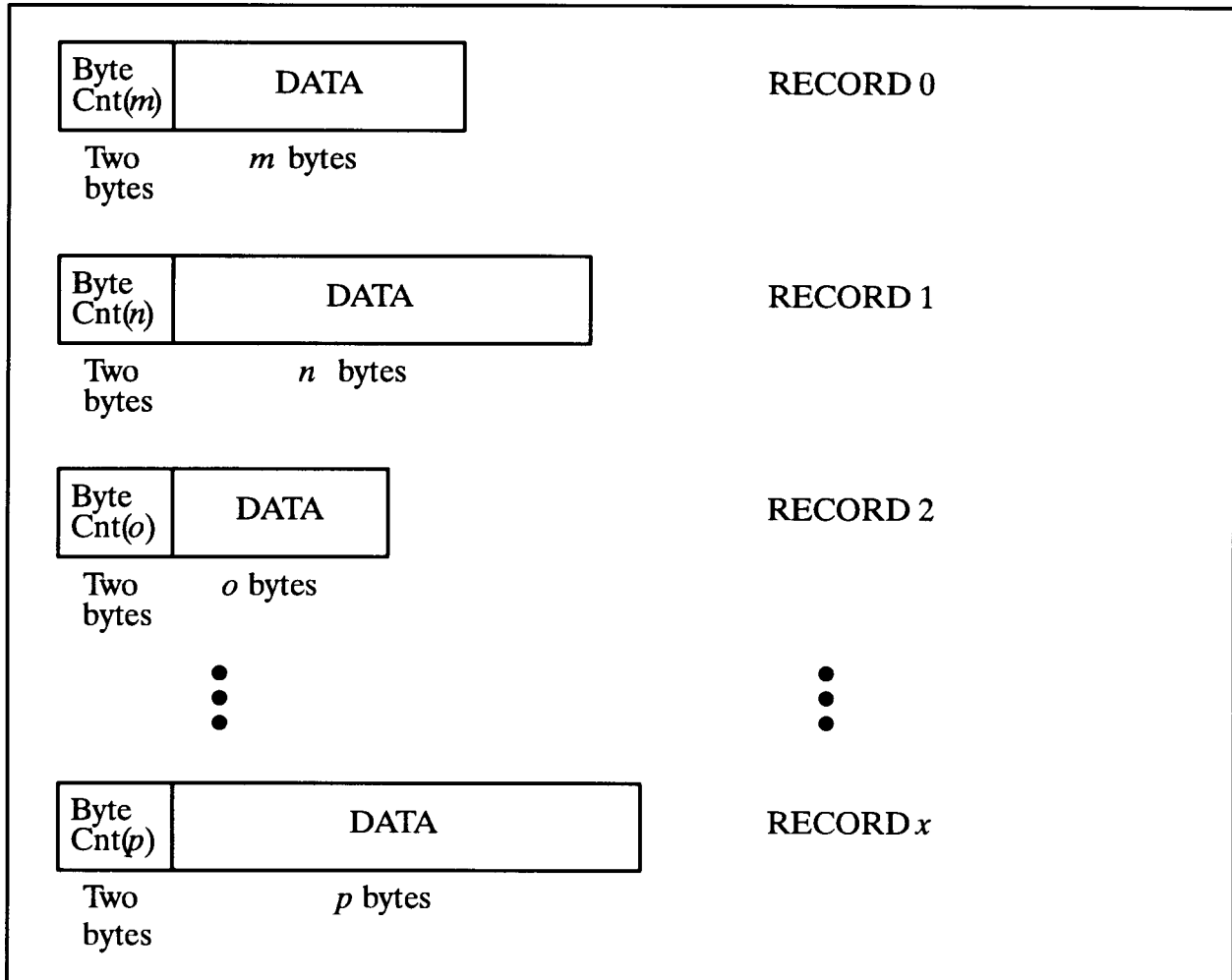
Figure 2-3. Variable-length Records
