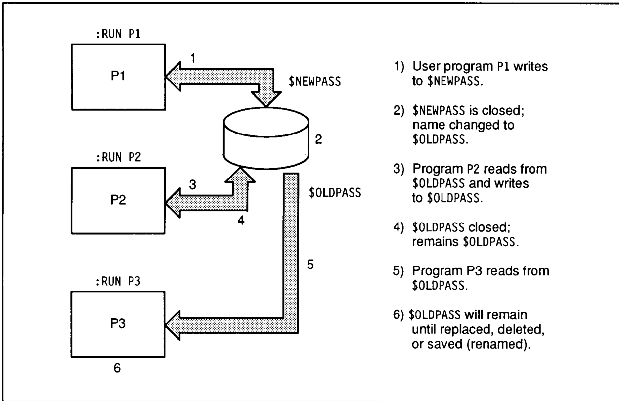
Figure 3-1. Passing Files between Program Runs
