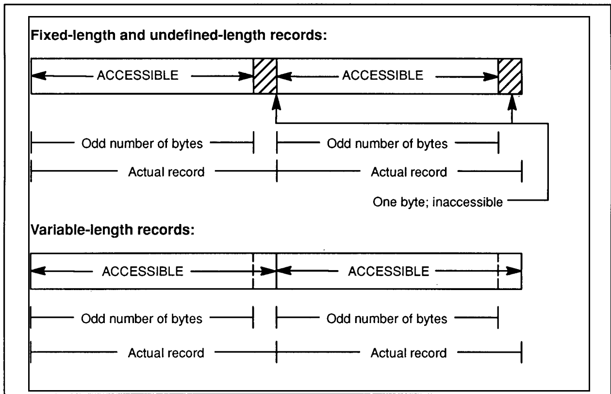
Figure 2-5. Record Placement for ASCII Files
