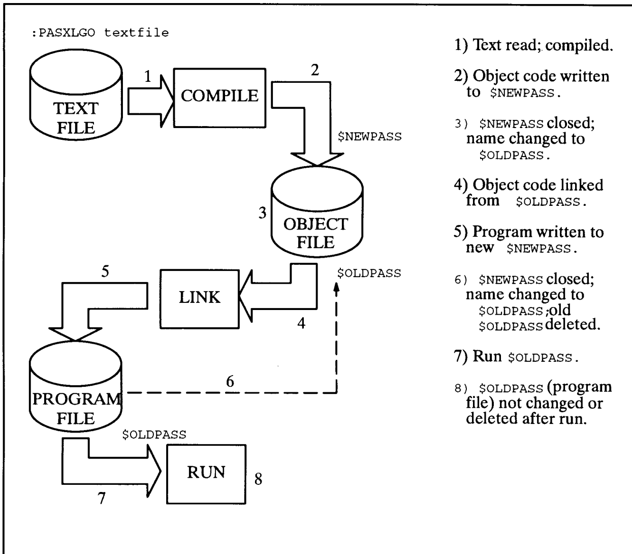
Figure 3-2. Passing Files within a Program Run
