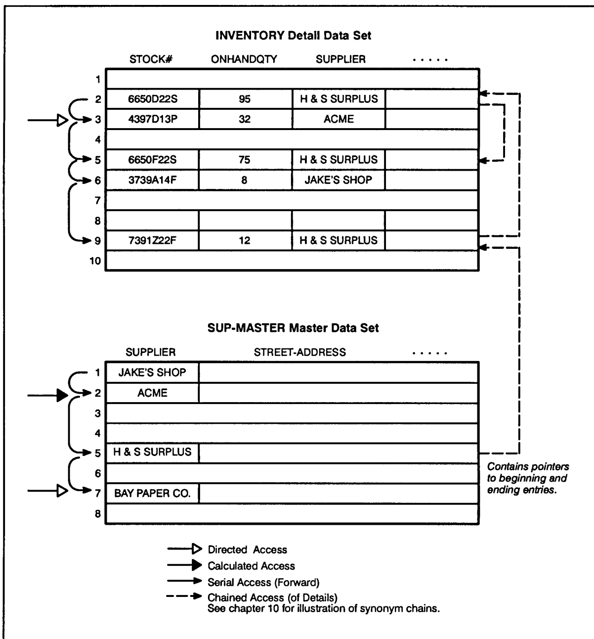
Figure 4-2. Reading Access Methods (DBGET Procedure)
