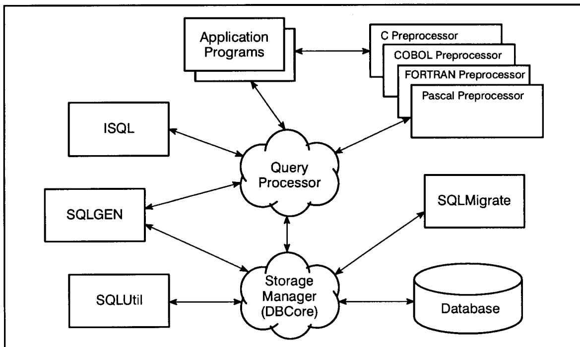
Figure 1-1. Components of ALLBASE/SQL
