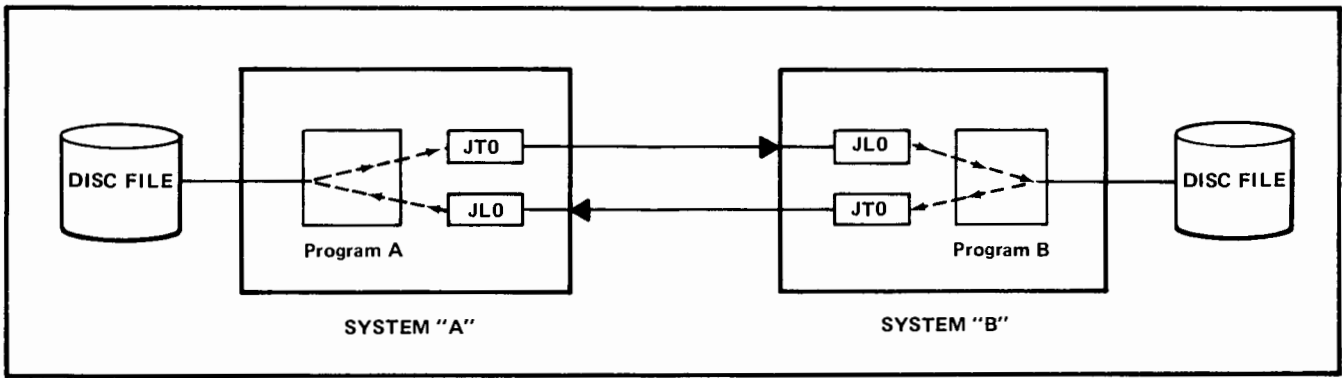
Figure 3. Transmitting Data Thru Job Transmitters/Listers
