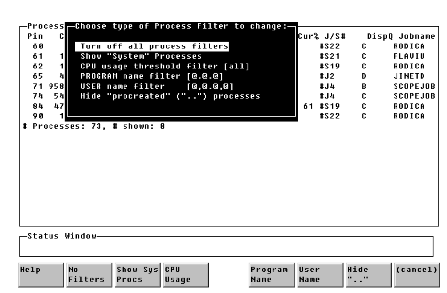
Figure 7.3 Process Action Pop-up Menu
