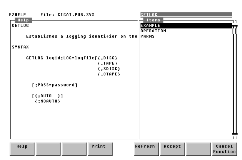
Figure 7.7 The Item Selection Window
