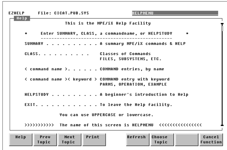
Figure 7.4 The System Help Display: Initial Screen
