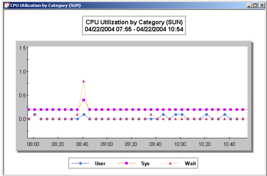
Figure 10.18 Example of CPU Utilization by Category Solaris Chart
