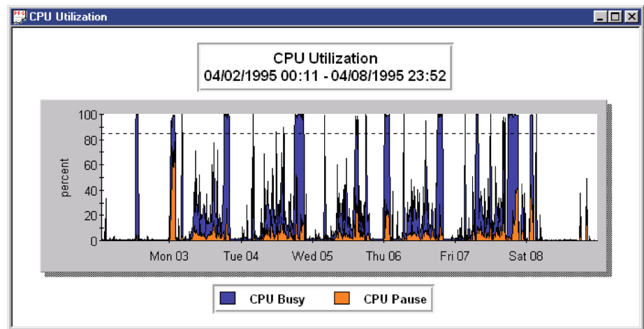
Figure 9.10 Example CPU Utilization (MPE) stacked area graph: CPU Pause
