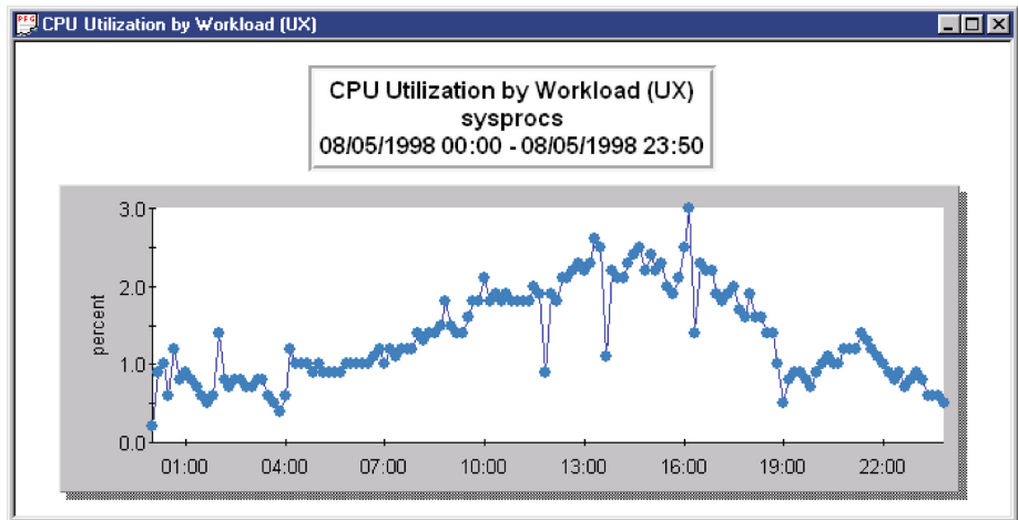
Figure 10.5 Example CPU Utilization by Workload (UX) subchart (sysprocs)
