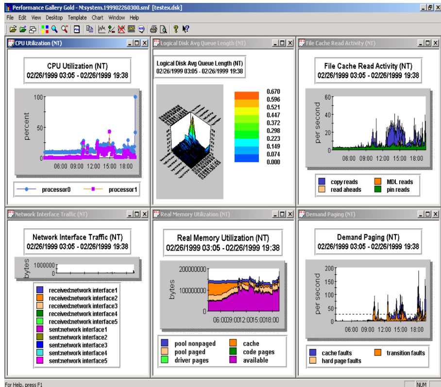
Figure 6.23 Example of active Performance Gallery Gold desktop
